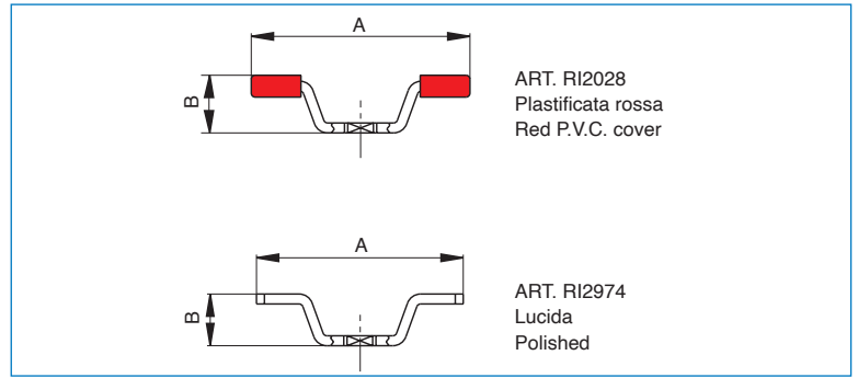
Farfalla in acciaio inox - Stainless steel butterfly handle - Papillon en acier inox - Flügelgriff aus Edelstahl - Mariposa en acero inox.
