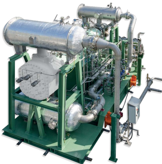
BOG compressor
